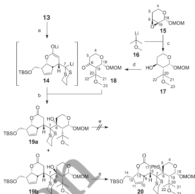
Scheme 4. Access to intermediate E through the synthesis of 20 .
