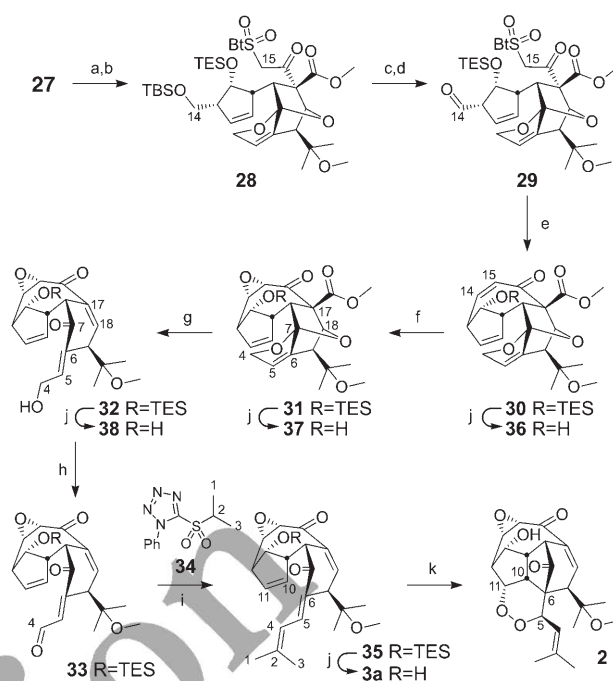
Scheme 6. Synthesis of desoxohexacyclinol ( 3 ). a) KHMDS (1.1 equiv), THF; -78^{\circ}\text{C} to -50^{\circ}\text{C} ; then (\text{BtS})_2 , -78^{\circ}\text{C} ; -78^{\circ}\text{C} \rightarrow 0^{\circ}\text{C} , 12 h; b) oxone, wet 1,4-dioxane, 87% from 27 ; c) TBAF, wet THF, 0^{\circ}\text{C} \rightarrow \text{RT} ; d) Dess–Martin periodinane, \text{CH}_2\text{Cl}_2 , 0^{\circ}\text{C} \rightarrow \text{RT} ; e) slow addition of DBU (1.2 equiv), DMAP (cat.), THF, -40^{\circ}\text{C} \rightarrow \text{RT} , 10 h, 72% from 28 ; f) Ph 3 COOH, L-(+)-diisopropyltartrate, toluene, \text{CH}_2\text{Cl}_2 (3:1 v/v), 92%; g) KOTMS, THF, -10^{\circ}\text{C} \rightarrow 35^{\circ}\text{C} , 5 h, 69%; h) \text{MnO}_2 , \text{CH}_2\text{Cl}_2 , room temperature; i) 34 , KHMDS, -78^{\circ}\text{C} ; -78^{\circ}\text{C} \rightarrow -30^{\circ}\text{C} , 2 h; add 33 at -78^{\circ}\text{C} ; -78^{\circ}\text{C} \rightarrow \text{RT} , 3 h; then room temperature, 12 h, 76% from 32 ; j) cat. aq. \text{H}_2\text{SiF}_6 , \text{CH}_3\text{CN}/t\text{BuOH} (9:1 v/v), room temperature, 78% for 3a ; 81% for 36 ; 72% for 37 ; 84% for 38 ; k) \text{O}_2 , rose bengal, MeOH, h\nu , 0^{\circ}\text{C} , 82%. Bt = 1-benzothiazole, TBAF = tetra- n -butylammonium fluoride, DBU = 1,8-diazabicyclo[5.4.0]undec-7-ene.
