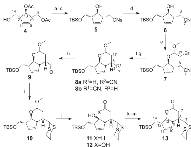
Scheme 3. Access to intermediate D through the synthesis of 13 .
